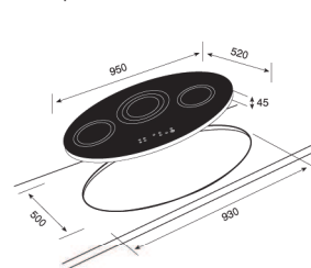
GKST-95 E D Select
