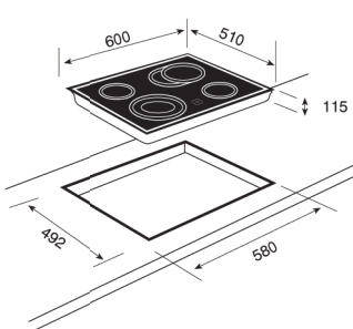
VTC-R 2DC E
